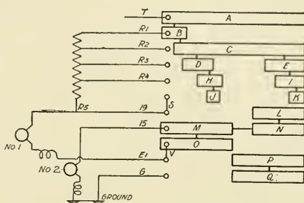
Fig. 53. Development of Controller Connections—Motors in Series
